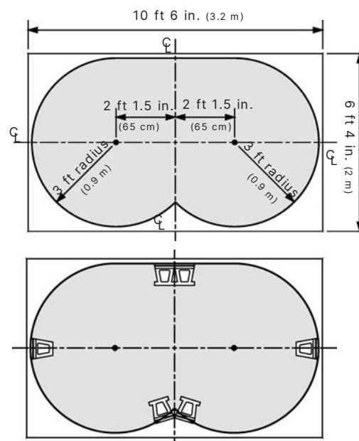
Remove Wings From Blocks
